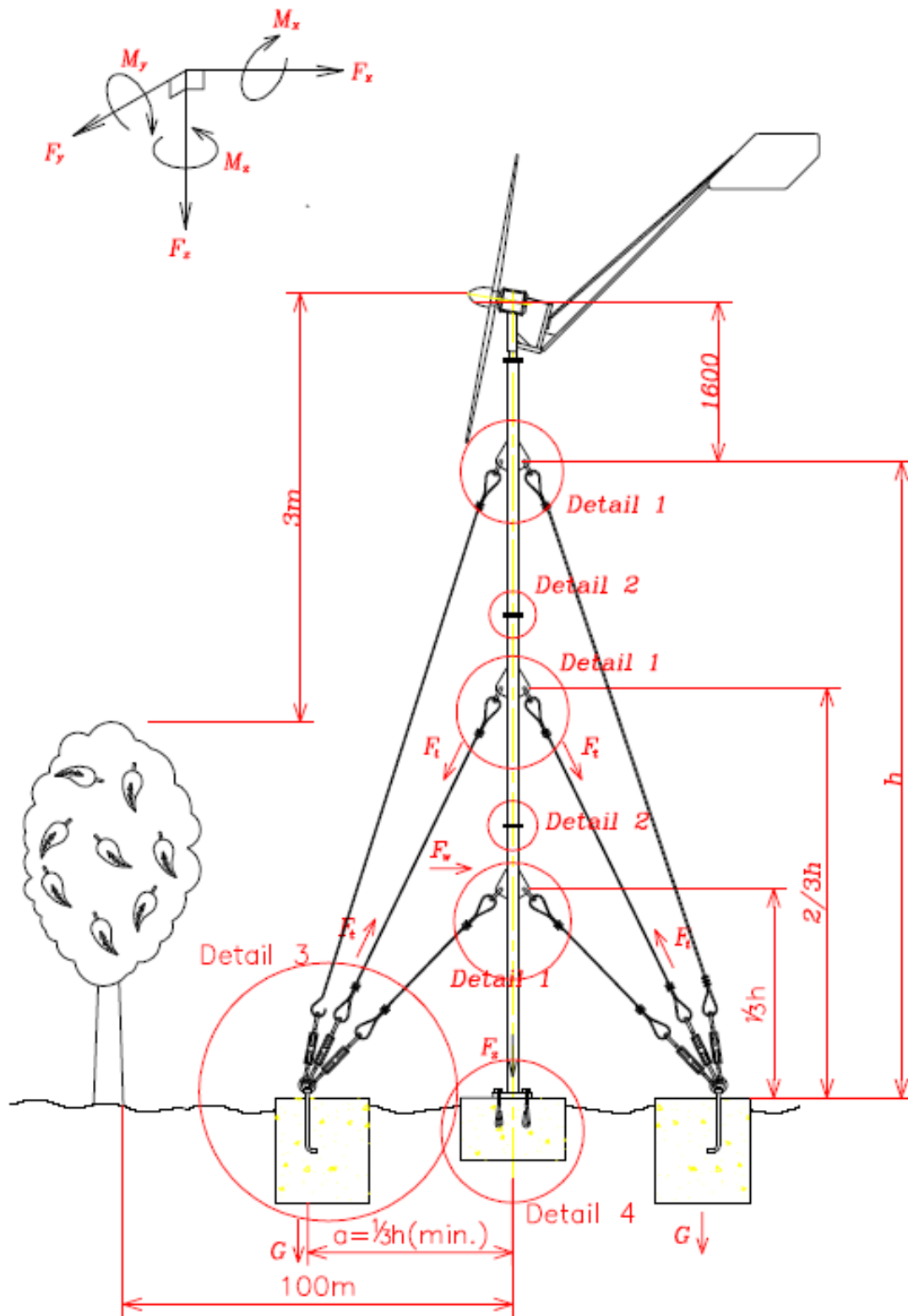
Guyed tower height 18 meter for Fortis Passaat 1.4 kW
